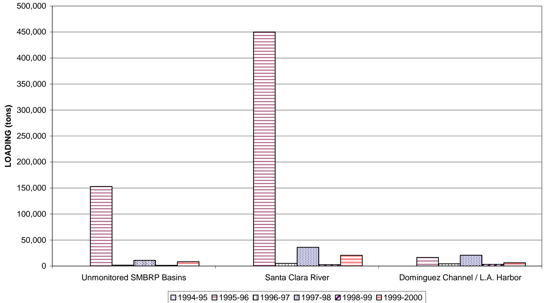
Figure 4-16a. TOTAL MASS EMISSION LOADINGS TOTAL SUSPENDED SOLIDS
