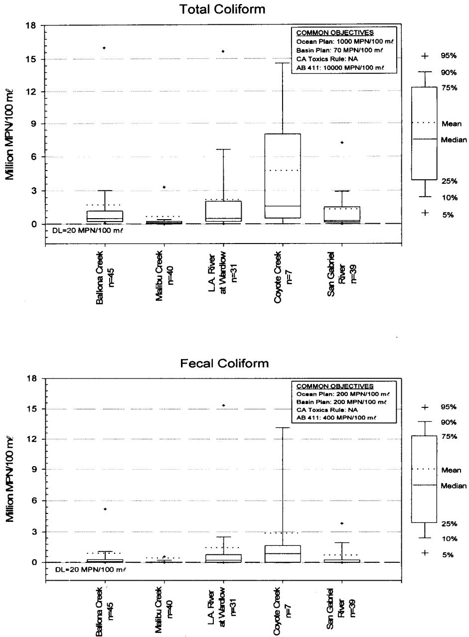
Mass Emission Box Plots 1994-2000 STORM SEASONS Figure 4-2
