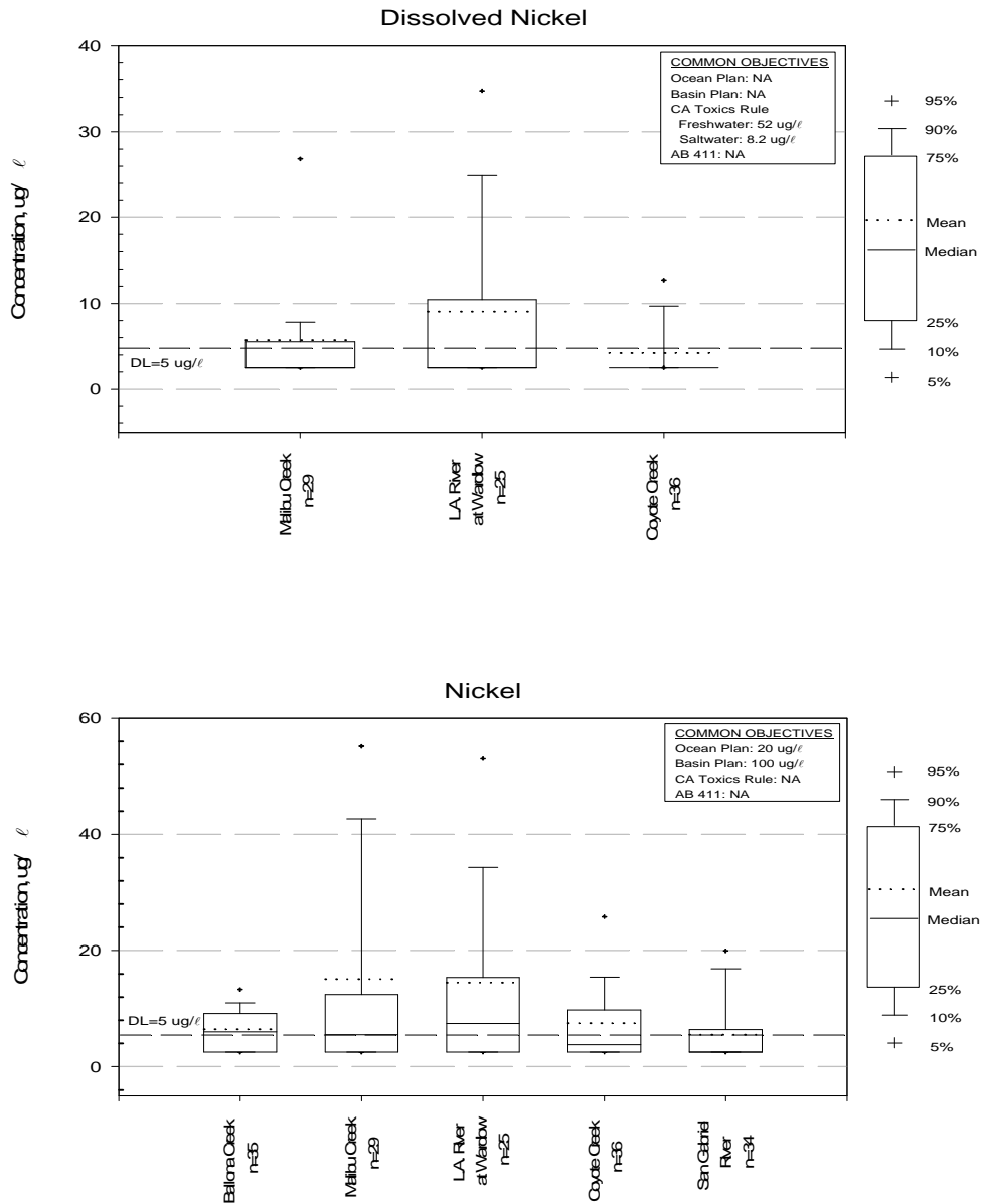
Mass Emission Box Plots 1994-2000 STORM SEASONS Figure 4-2
