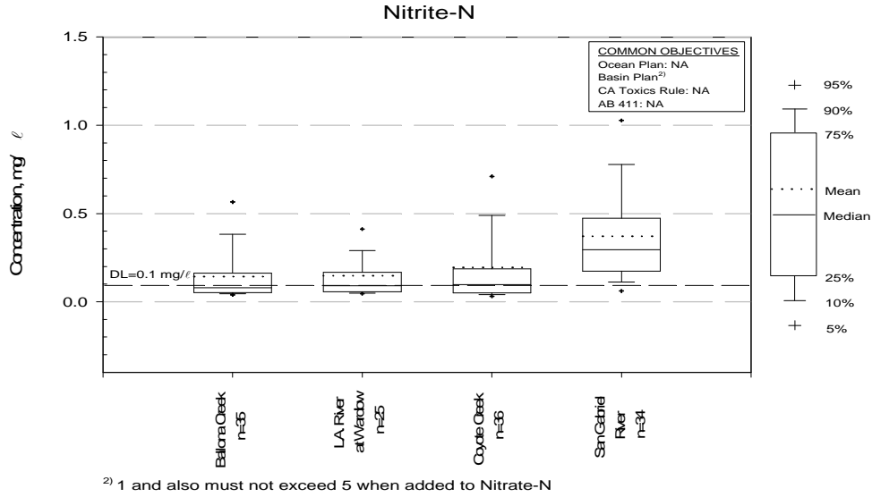
Mass Emission Box Plots 1994-2000 STORM SEASONS Figure 4-2
