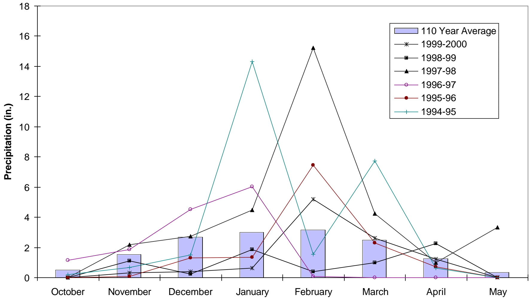
Figure 4-21 Historic Los Angeles Monthly Wet Season Rainfall at Station #716, Ducommun St., Los Angeles
