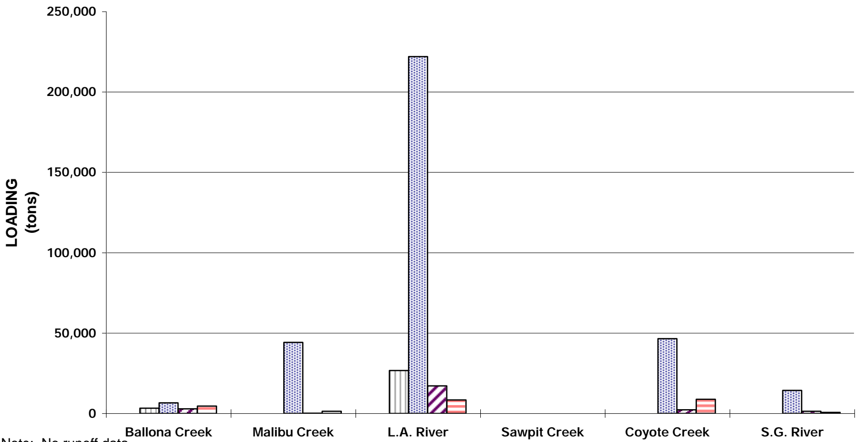
Figure 4-5a. MASS EMISSION LOADINGS TOTAL SUSPENDED SOLIDS
